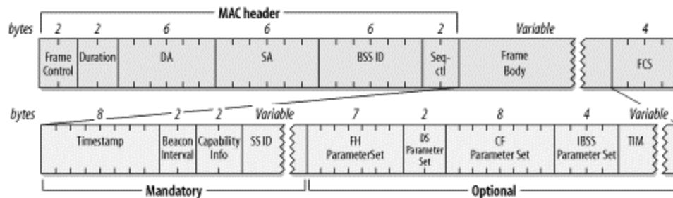
Figure 4-39. Beacon frame
