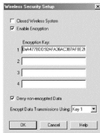
Figure 14-7. WEP configuration dialog box
