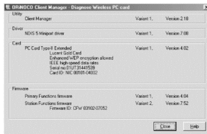
Figure 12-33. Version information
