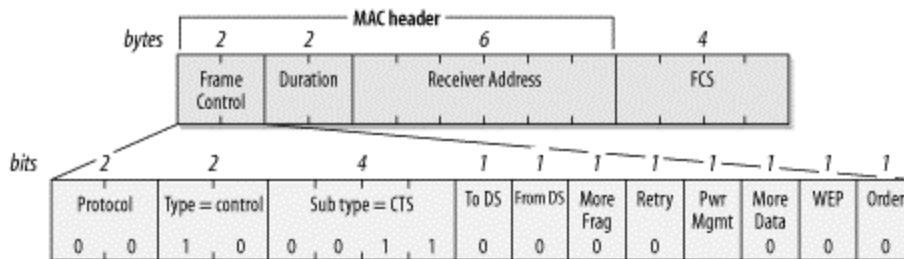
Figure 4-15. CTS frame
