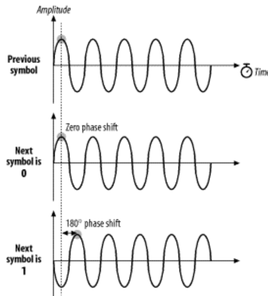
Figure 10-19. DBPSK encoding
