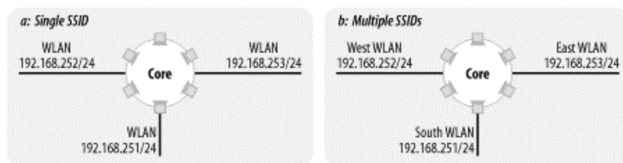
Figure 15-4. Noncontiguous deployments
