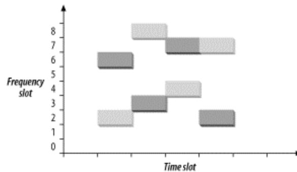
Figure 10-3. Orthogonal hopping sequences
