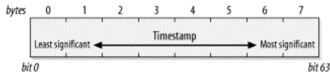
Figure 4-28. Timestamp field
