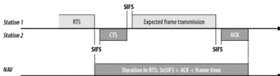
Figure 4-14. Duration field in RTS frame
