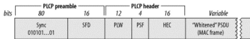
Figure 10-9. PLCP framing in the FH PHY
