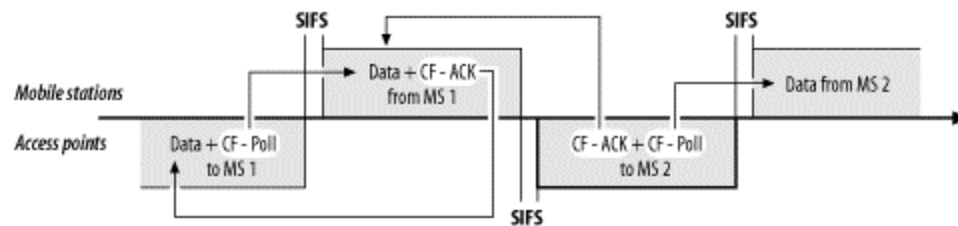
Figure 8-6. CF-Ack+CF-Poll usage
