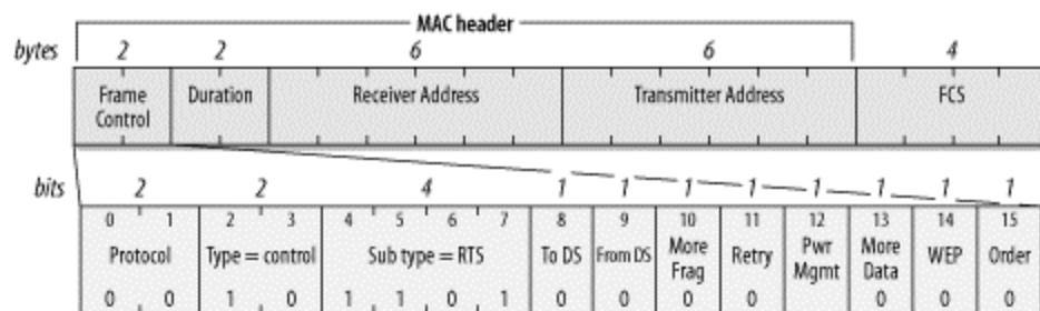
Figure 4-13. RTS frame
