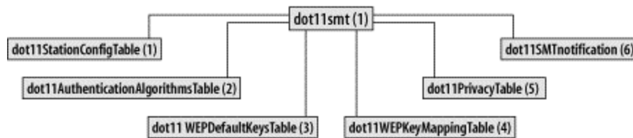
Figure A-2. Main branches of the station management (SMT) tree
