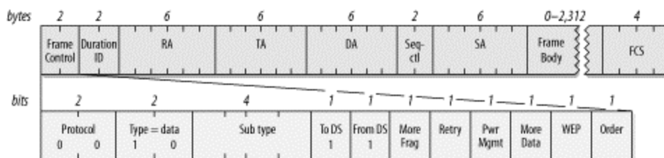
Figure 4-11. WDS frames
