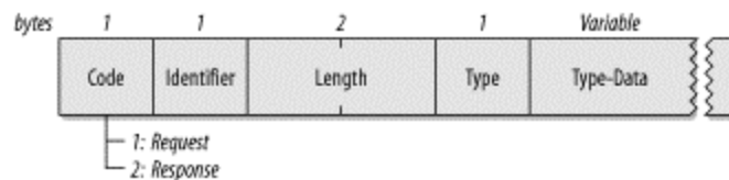
Figure 6-3. EAP Request and EAP Response packets
