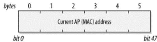
Figure 4-25. Current AP Address field
