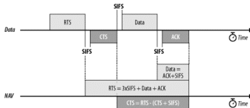
Figure 3-17. RTS/CTS lockout
