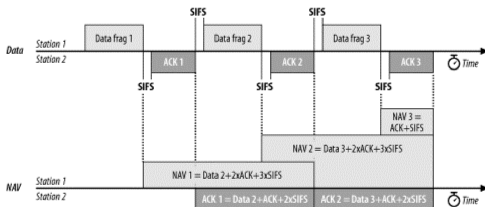
Figure 3-16. Fragmentation
