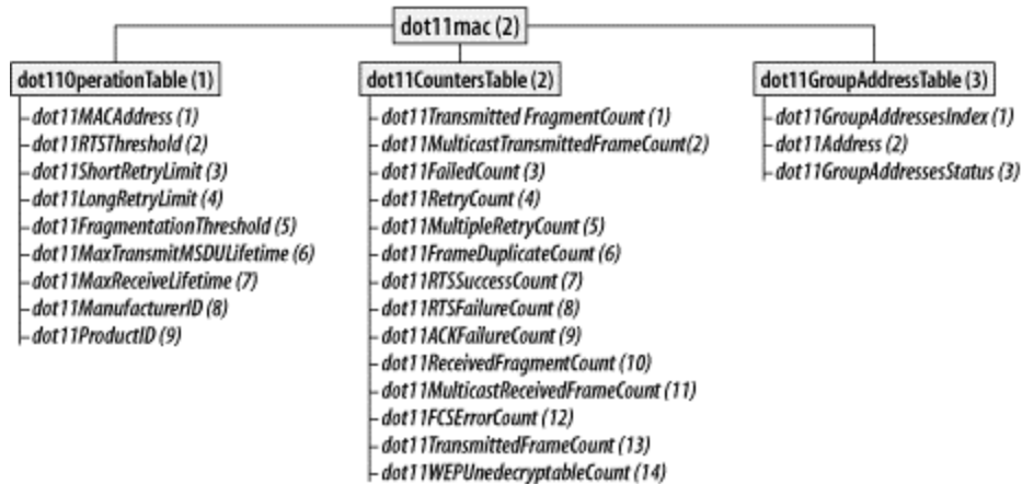
Figure A-6. The MAC attributes subtree
