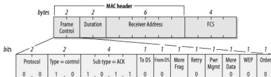
Figure 4-17. ACK frame
