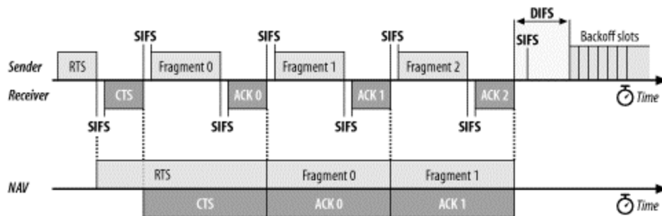
Figure 3-8. Fragmentation burst
