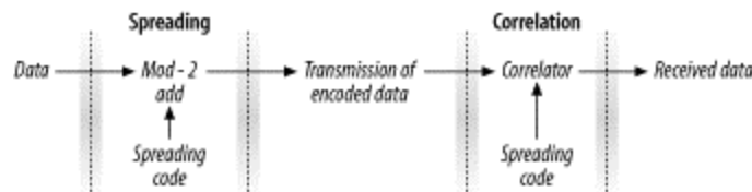
Figure 10-13. Chipping
