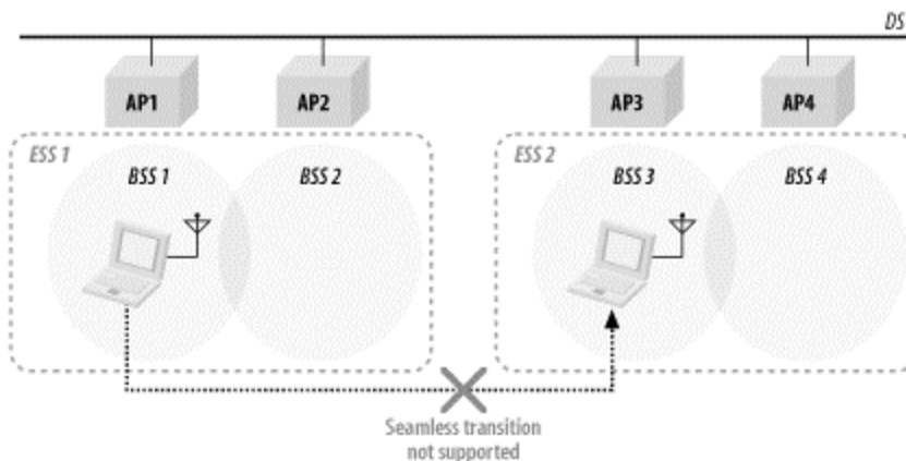
Figure 2-10. ESS transition
