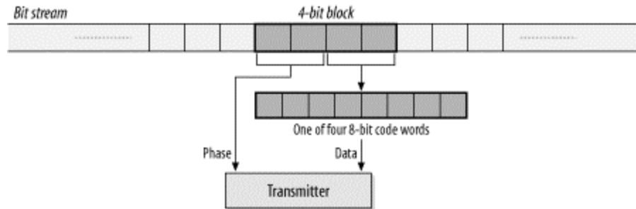
Figure 10-29. 802.11b transmission at 5.5 Mbps
