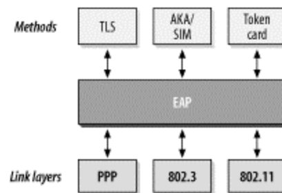
Figure 6-1. EAP architecture
