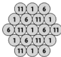
Figure 15-6. Frequency planning
