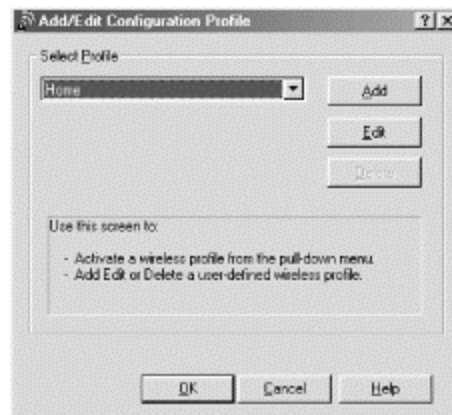
Figure 12-26. Profile creation
