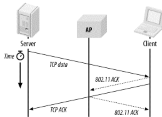
Figure 16-26. Frames corresponding to the bulk transfer of an HTTP connection
