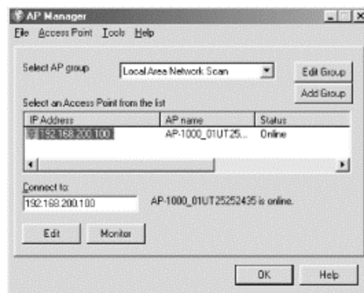
Figure 14-1. AP list
