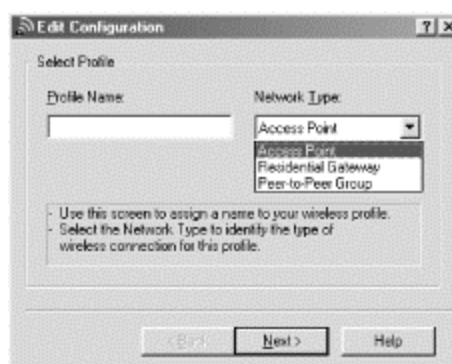
Figure 12-26. Profile creation
