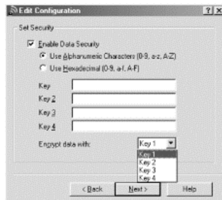
Figure 12-29. WEP configuration
