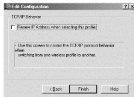
Figure 12-31. Network control
