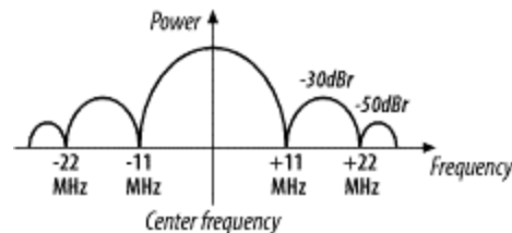
Figure 10-15. Energy spread in a single 802.11 DS transmission channel
