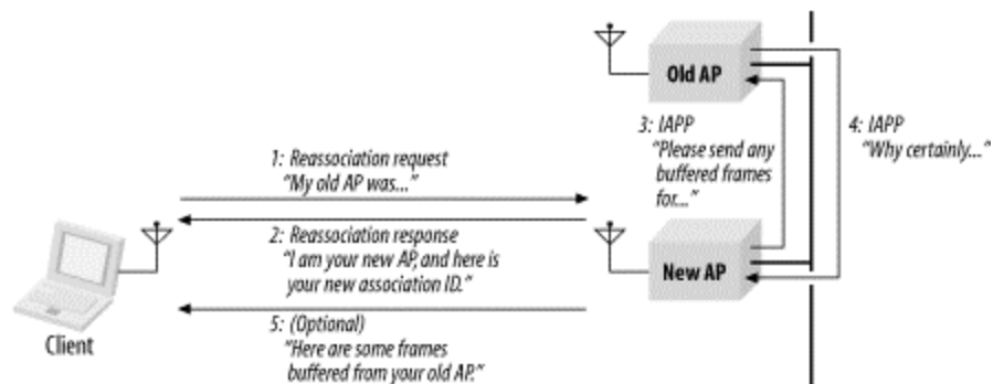
Figure 7-8. Reassociation procedure
