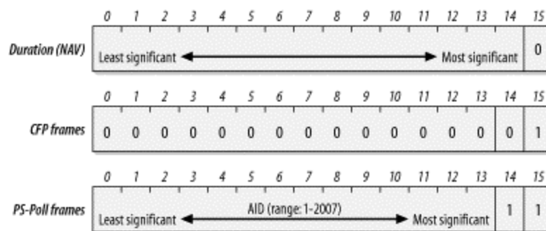
Figure 3-11. Duration/ID field
