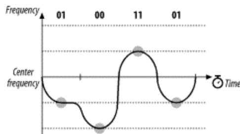
Figure 10-8. 4GFSK encoding of the letter M
