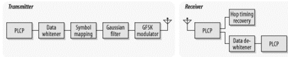
Figure 10-10. Frequency-hopping transceiver
