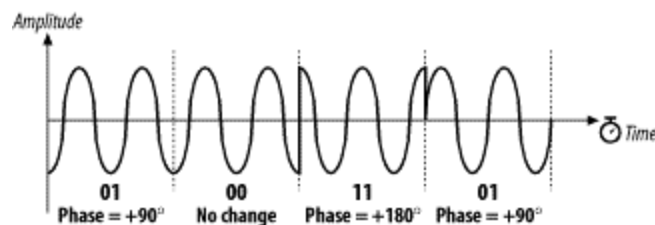
Figure 10-22. The letter M encoded in DQPSK
